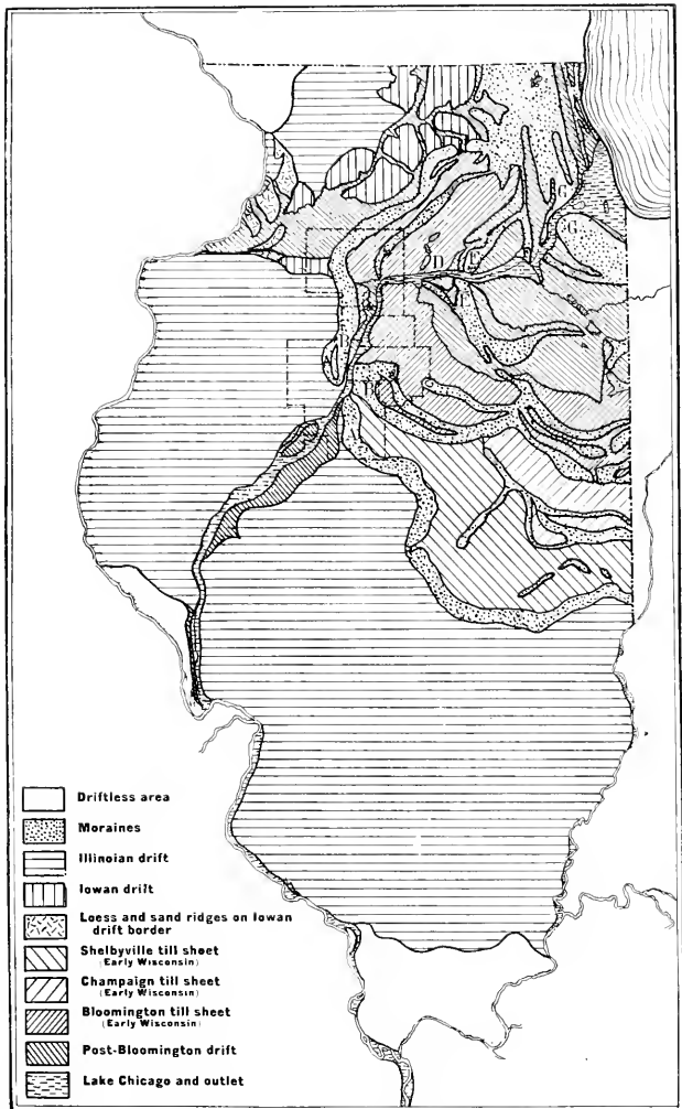
FIG. 20. Generalized glacial map of Illinois. (Data from Leveitt's map, Monograph 38, U. S. Geol. Surv.)
